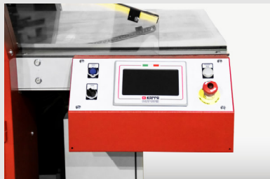
Touch panel 7"
